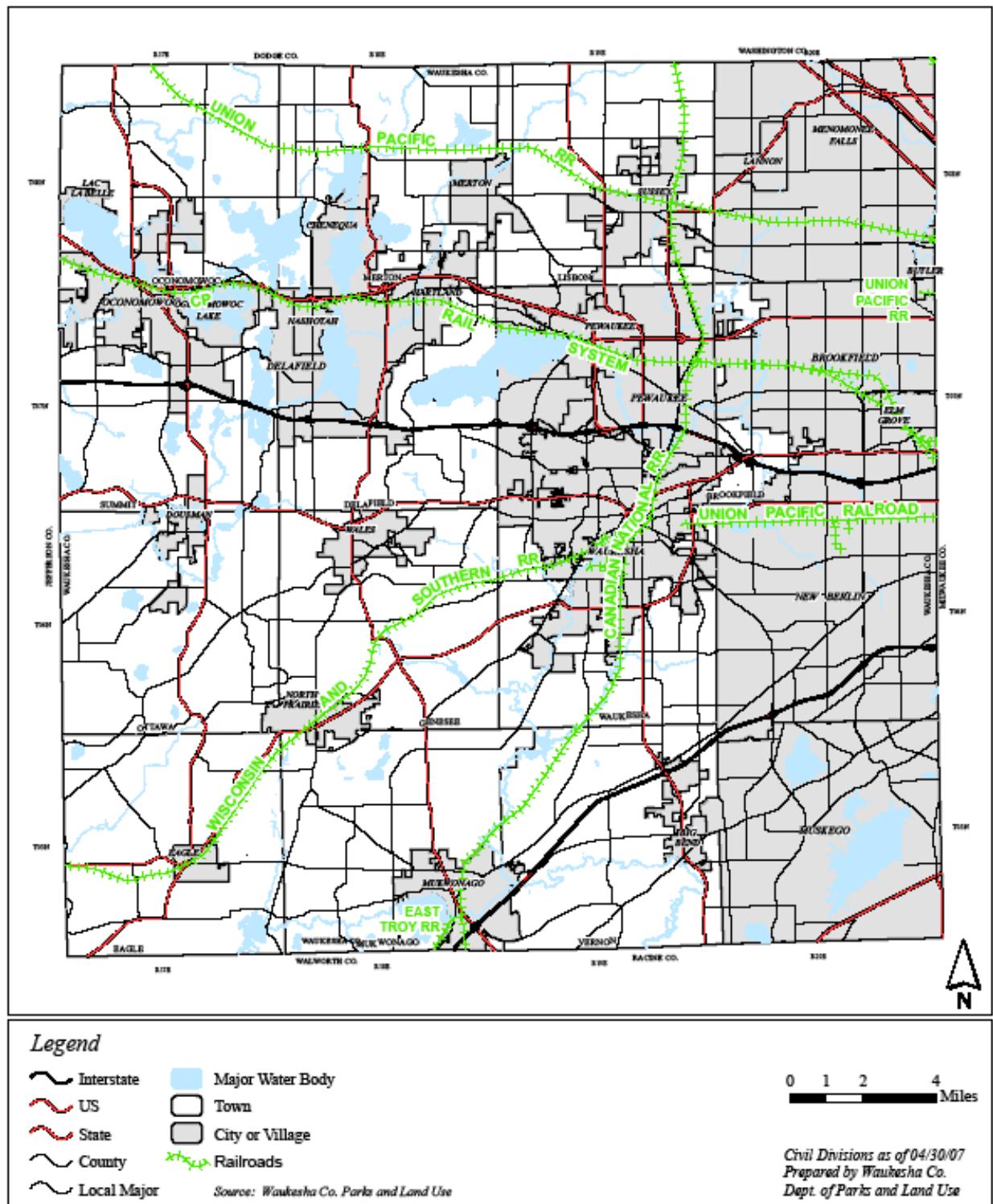
Map VIII-3 Existing Railroad Routes in Waukesha County: 2007
